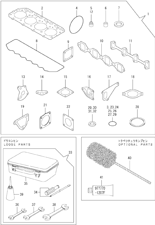
Fig.18. GASKET SET & TOOLS
