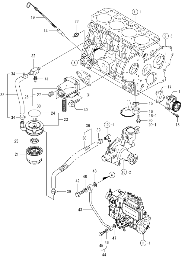
Fig.9. LUB.OIL SYSTEM
