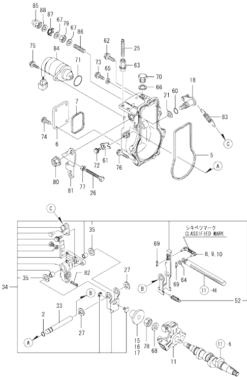
Fig.12. GOVERNOR
